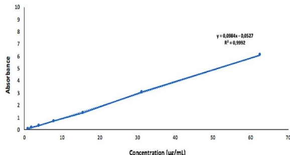
Fig. 8: Ciprofloxacin calibration graph.
